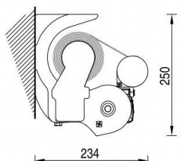
Ceiling installation
