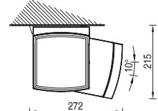
Ceiling installation 65°
