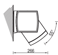
Wall installation 55°
