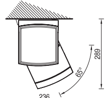
Ceiling installation 65°
