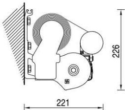
Wall installation
