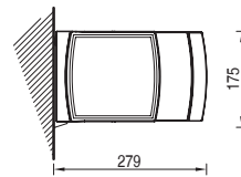
Wall installation 55°
